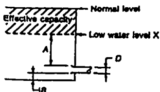
(b) Storage with side suction pipe
